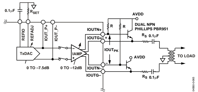
Figure 65. Voltage-Mode Operation
